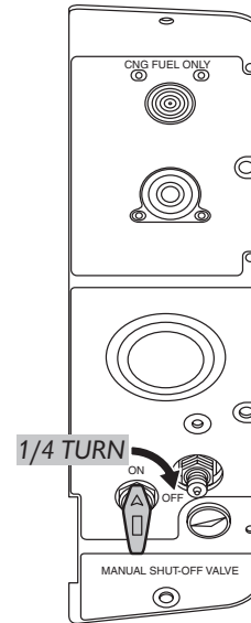
FIGURE 2 – FMM MANUAL SHUT-OFF VALVE
