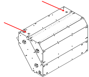
FIGURE 16 – TAIL MOUNT VENT PORTS
