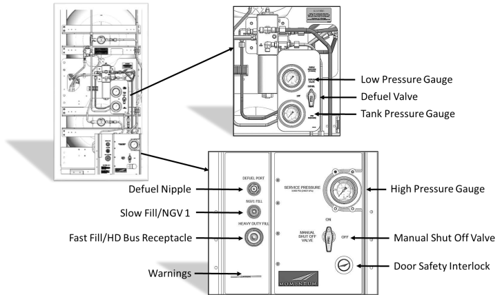
FIGURE 10 – FUEL MANAGEMENT MODULE
