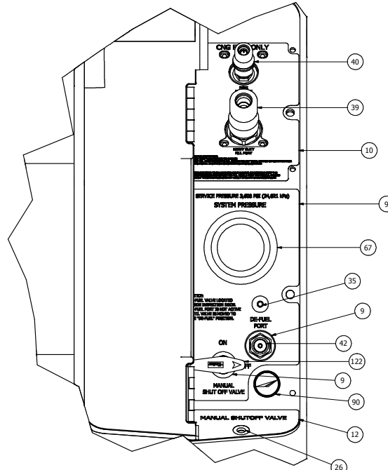
DETAIL C SCALE 1/2
