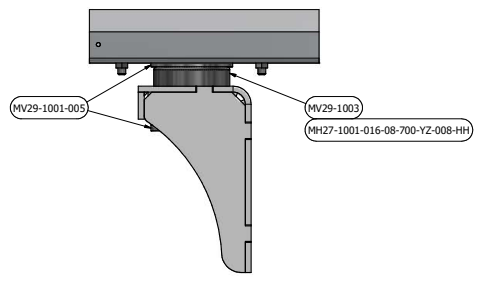
DETAIL A SCALE 1/4
