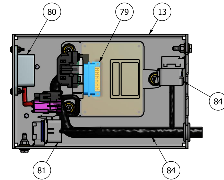
SECTION A-A SCALE 1 / 3
