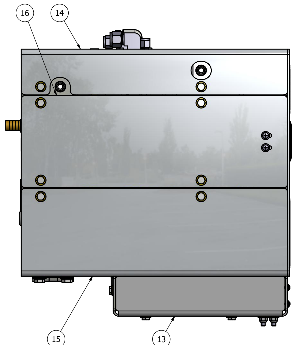
SIDE VIEW
