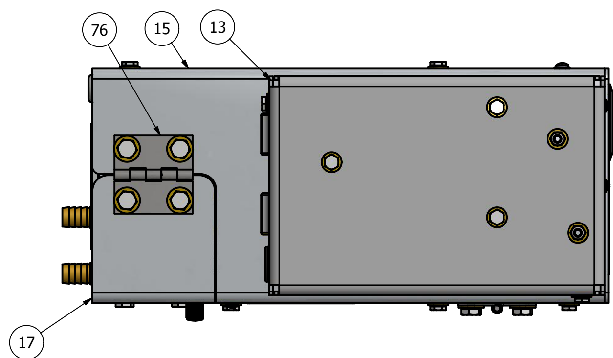
BOTTOM VIEW
