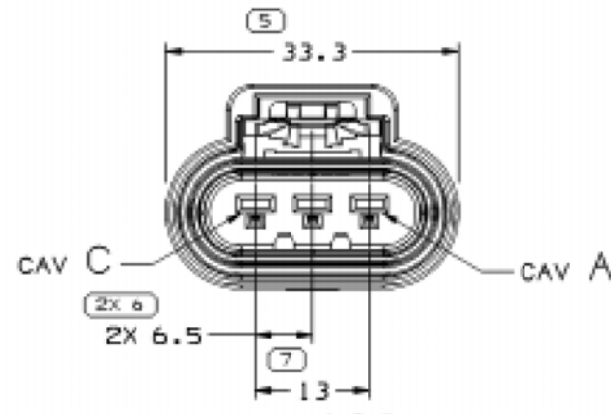
P1 FUEL SENDER, SENDER SIDE DELPHI 12110293
