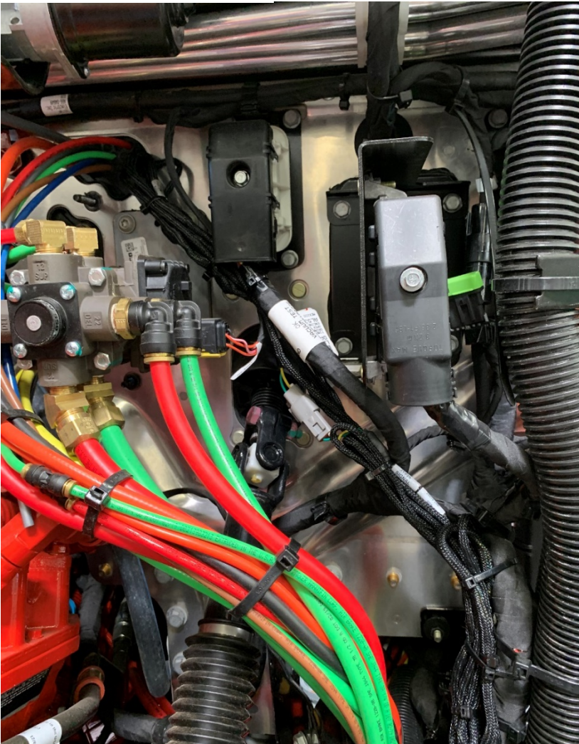
Figure 18: Under Hood Wiring
