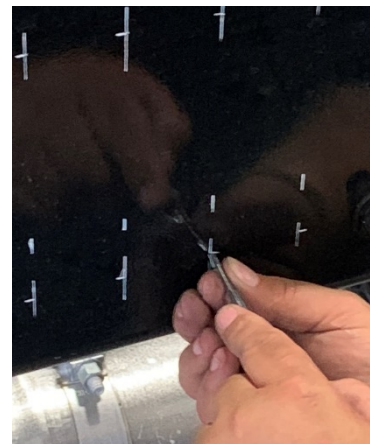
Figure 7: Center Punching Holes
