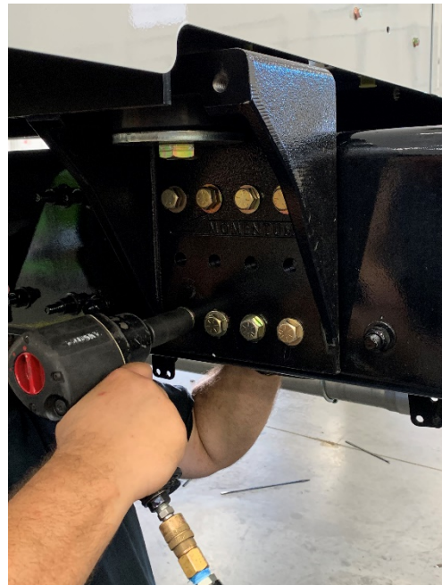
Figure 32: Torquing Mounting Bolts
