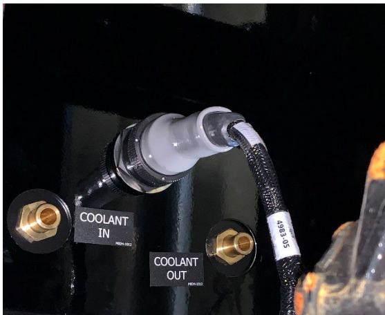
Figure 34: BOC Electrical Connection
