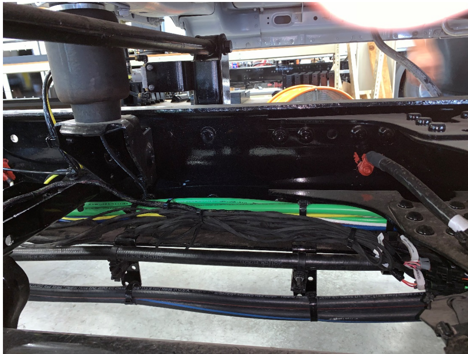
Figure 15: Wiring Harness Routing-Behind Cab
