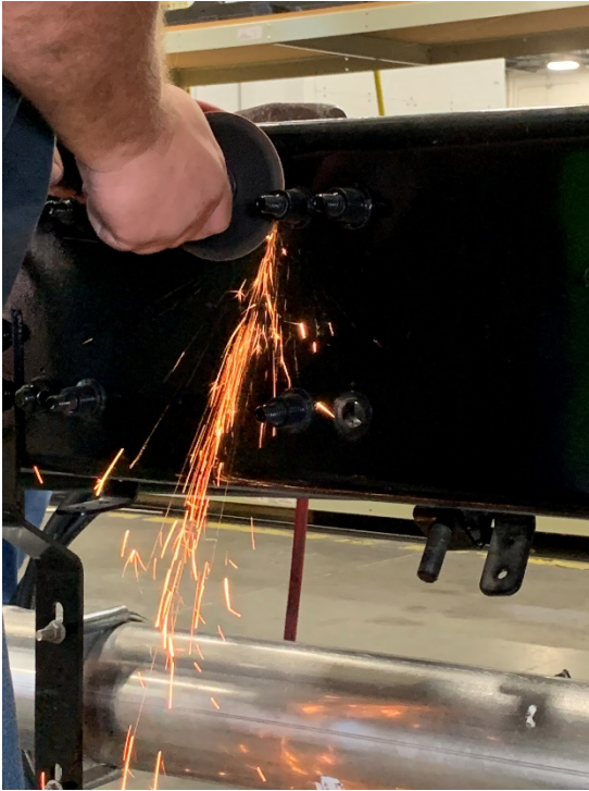
Figure 6: Cutting Huck Bolt
