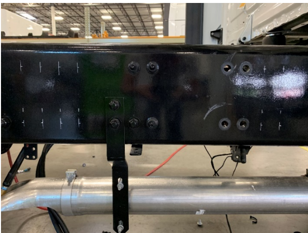
Figure 8: Marked Holes on Chassis
