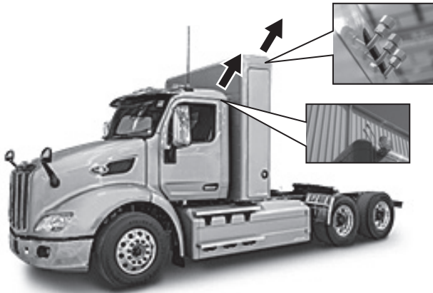
FIGURE 10 – VENT PORTS AND VENT CAPS
