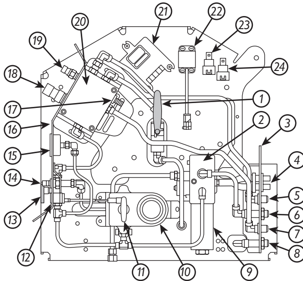
FIGURE 17 – CNG COMPONENTS
