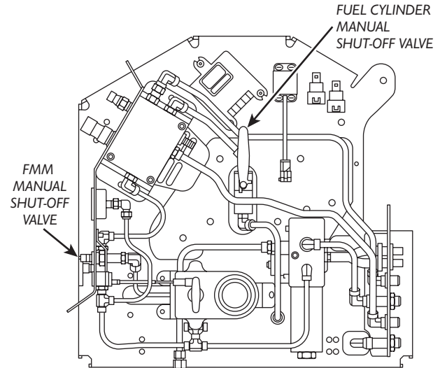
FIGURE 1 - MANUAL SHUT-OFF VALVES
