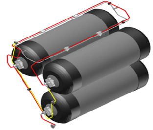
FIGURE 16 – TAIL MOUNT VENT PORTS
