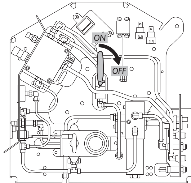
FIGURE 3 – CYLINDER MANUAL SHUT-OFF VALVE
