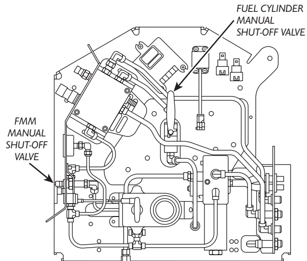
FIGURE 1 – MANUAL SHUT-OFF VALVES
