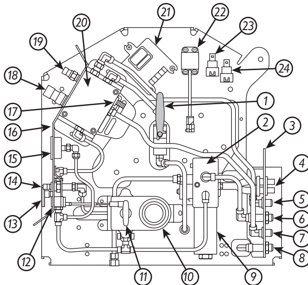
FIGURE 17 – CNG COMPONENTS
